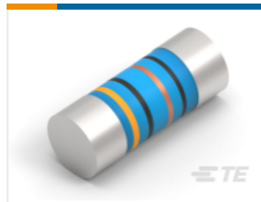
TE Model / Part #3-2176314-8 MELF SMA_A 180R 1% 50PPM 0102 0.3 W
